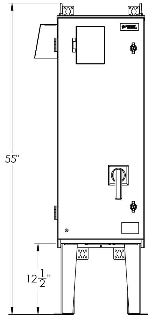
SHOWN WITH OPTIONAL LEG KIT AND MCCB
